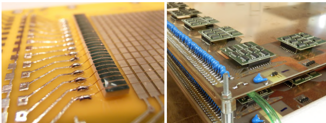
Figure 2.6: One of the gaseous detectors developed by the REGARD group[50]. Left: the inner structure contains wires which provide the coordinate information of the passing particle. Right: photo from the assembled detector, containing the custom designed electronics and a gas inlet tube (green).
