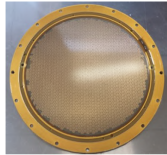
Figure 3.32: The Micromegas base of a borehole TPC from the CEA team [112].
