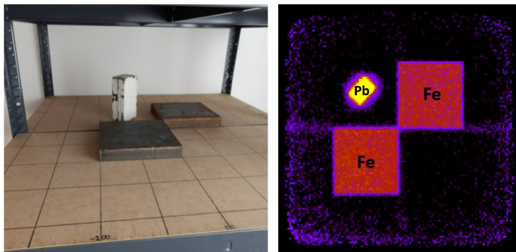
Figure 2.5: First scattering muography image of two Fe and a Pb blocks from our research group in Wigner RCP [39].
