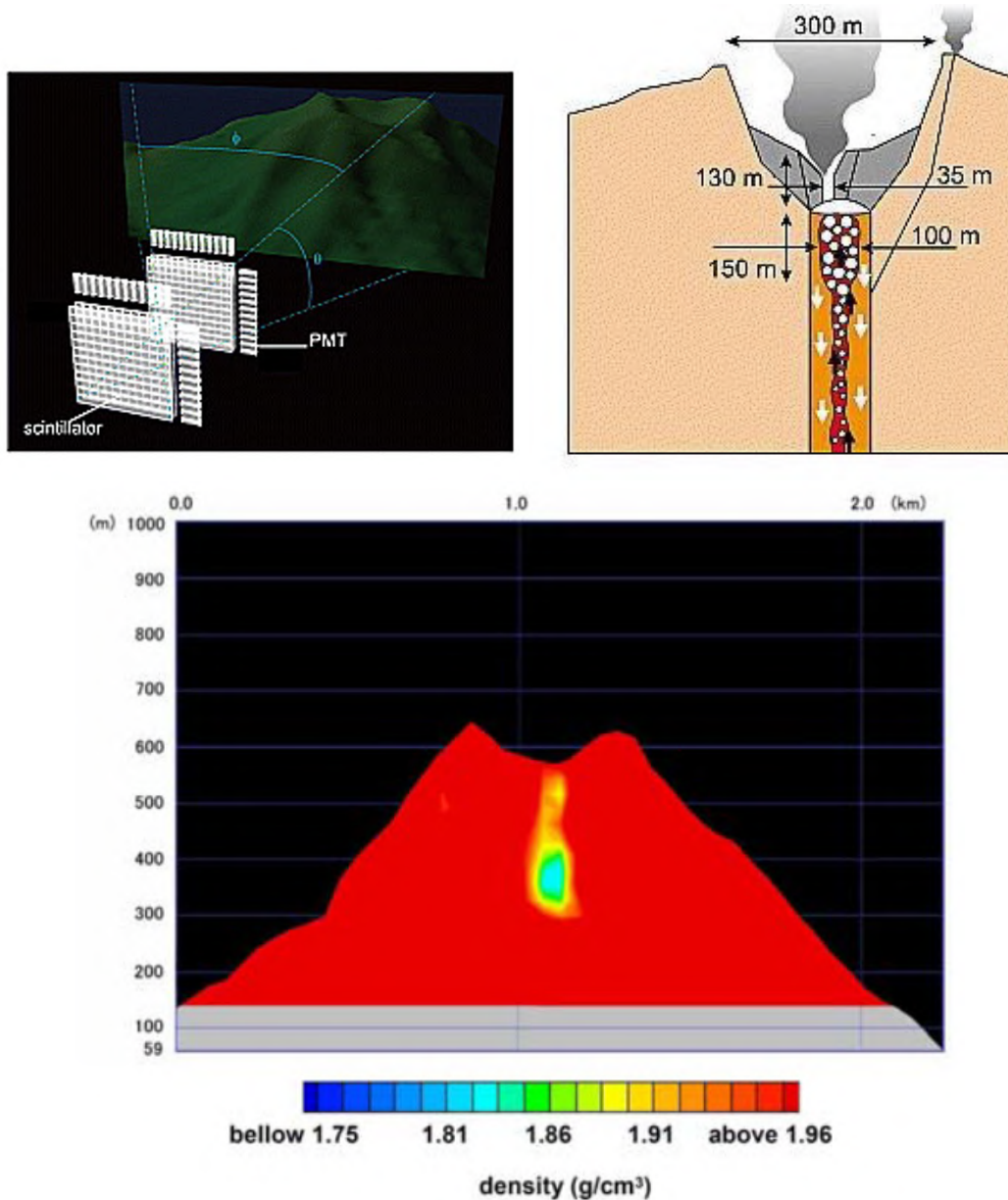
Figure 2.4: The schematic view of the interior structure of the Satsuma-Iwojima Volcano (top right) and the muography detection principle (top left). The resulting muographic density image of the upper few hundred meters of the volcanic cone (bottom) [6].
