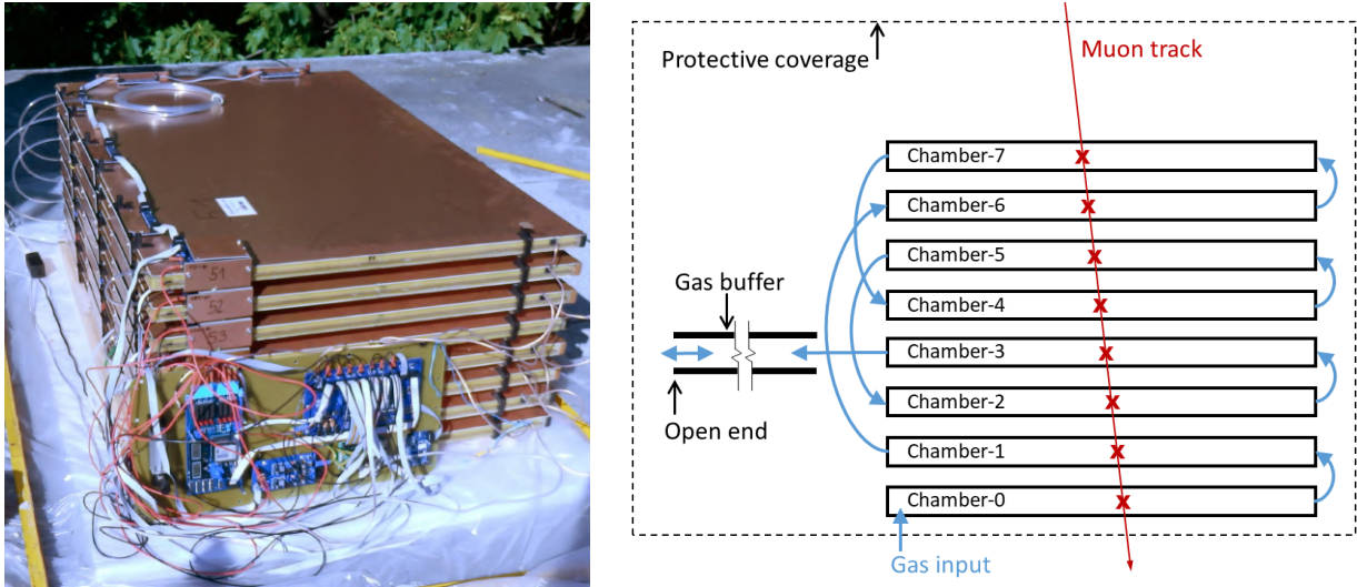
Figure 3.16: Left: The measurement setup installed outdoor, with protective coverage removed. The structure is the same as the one used for outgassing tests in the laboratory conditions. Right: Scheme showing the detector setup with eight MWPC chambers. The gas flows serially through the chambers according to the blue arrows, followed by a buffer tube with open end [98].
