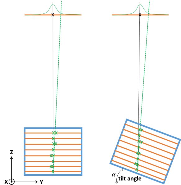
Figure 3.14: Sketch of the direct measurement of angular resolution for tracking detectors.
